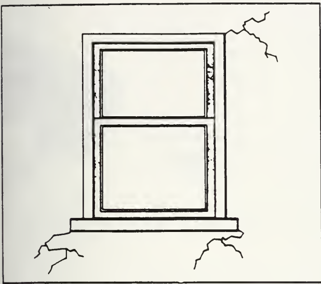
Fig. 1.4—Typical crack patterns at reentrant corners (Reference 2)
